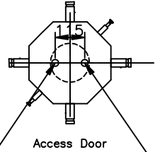
Top Entry (CWTT) Connection Details ( Viewed from Above )
