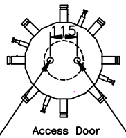
Top Entry (CWTT) Connection Details ( Viewed from Above )
