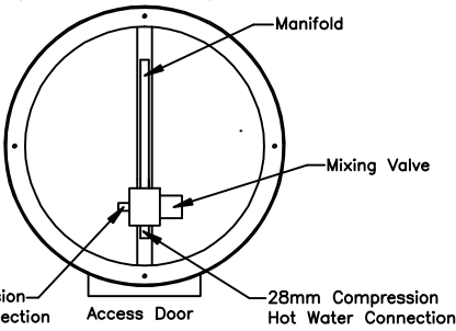
Bottom Entry (CWTB) Connection Details ( Viewed from Below )
